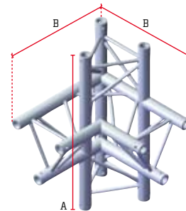
4 WAYCORNER 90° LEFT
