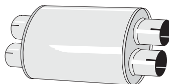
U 34 51 DR Ljuddämpare/silencer "DUO 51" Rör/pipe dimensions: 4x50,8 mm Oval 115/185 mm, L=315 mm (excl. muffar/ends)
