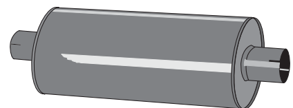
U 33 51 39 Ljuddämpare/Silencer "MEDIUM 51" Oval 100/165 mm L=420 mm (excl. muffar/ends)
