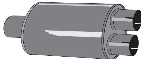
U 34 76 63 Ljuddämpare/silencer "SPLIT 76" Rör/pipe dimensions: 76 mm + 2x63,5 mm Oval 140/220 mm, L=320 mm (excl. muffar/ends)
