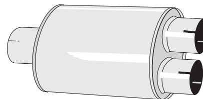
U 34 76 63R Ljuddämpare/silencer "SPLIT 76" Rör/pipe dimensions: 76 mm + 2x63,5 mm Oval 140/220 mm, L=320 mm (excl. muffar/ends)
