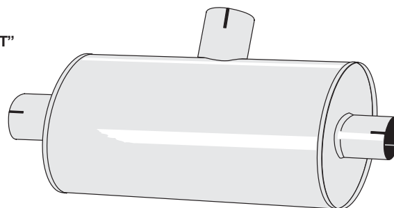
U 32 76 63R Ljuddämpare/Silencer "DUPLEX 76-63" Rör/pipe dimensions: 76 mm + 2x63,5 mm Oval 140//220 mm, L=500 mm (excl. muffar/ends)
