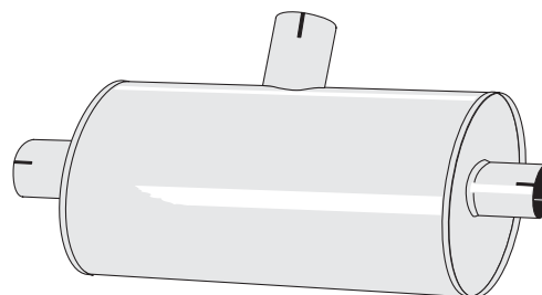
U 32 63 51R Ljuddämpare/Silencer "DUPLEX 63-51" Rör/pipe dimensions: 63,5 mm + 2x50,8 mm Oval 140/220 mm, L=500 mm (excl. muffar/ends)
