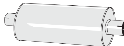
U 33 51 00R Ljuddämpare/Silencer "MEDIUM 51" Oval 100/165 mm, L=420 mm (excl. muffar/ends)
