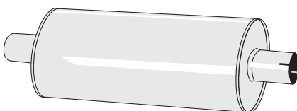
U 33 45 00R Ljuddämpare/Silencer "MEDIUM 45" Oval 100/165 mm, L=420 (excl. muffar/ends)
