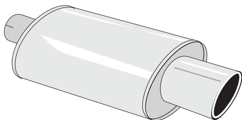
U 22 63 01R Slutdämpare/Rear silencer "ELLIPS 63" Oval 140/165 mm, L=420 (excl. muffar/ends) Totallängd/total length = 670 mm (incl. ändrör/tailpipe) Ändrör/tailpipe: 90/120 mm, snett/skewed Med upphängningsögla/With hanging point.
