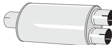
U 34 63 51R Ljuddämpare/silencer "SPLIT 63" Rör/pipe dimensions: 63,5 mm + 2x50,8 mm Oval 115/185 mm, L=320 mm (excl. muffar/ends)
