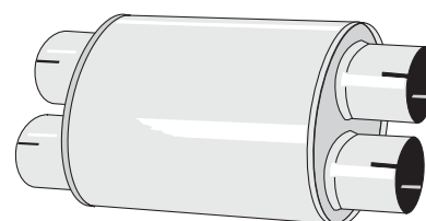
U 34 76 DR Ljuddämpare/silencer "DUO 76" Rör/pipe dimensions: 4x76 mm Oval 140/220 mm, L=315 mm (excl. muffar/ends)
